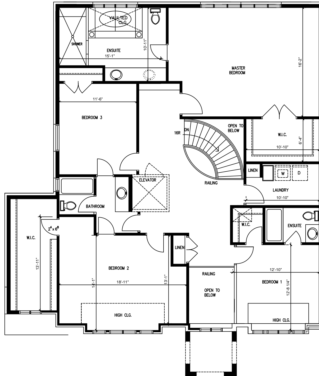
2ND FLOOR PLAN 2057 S.F.
