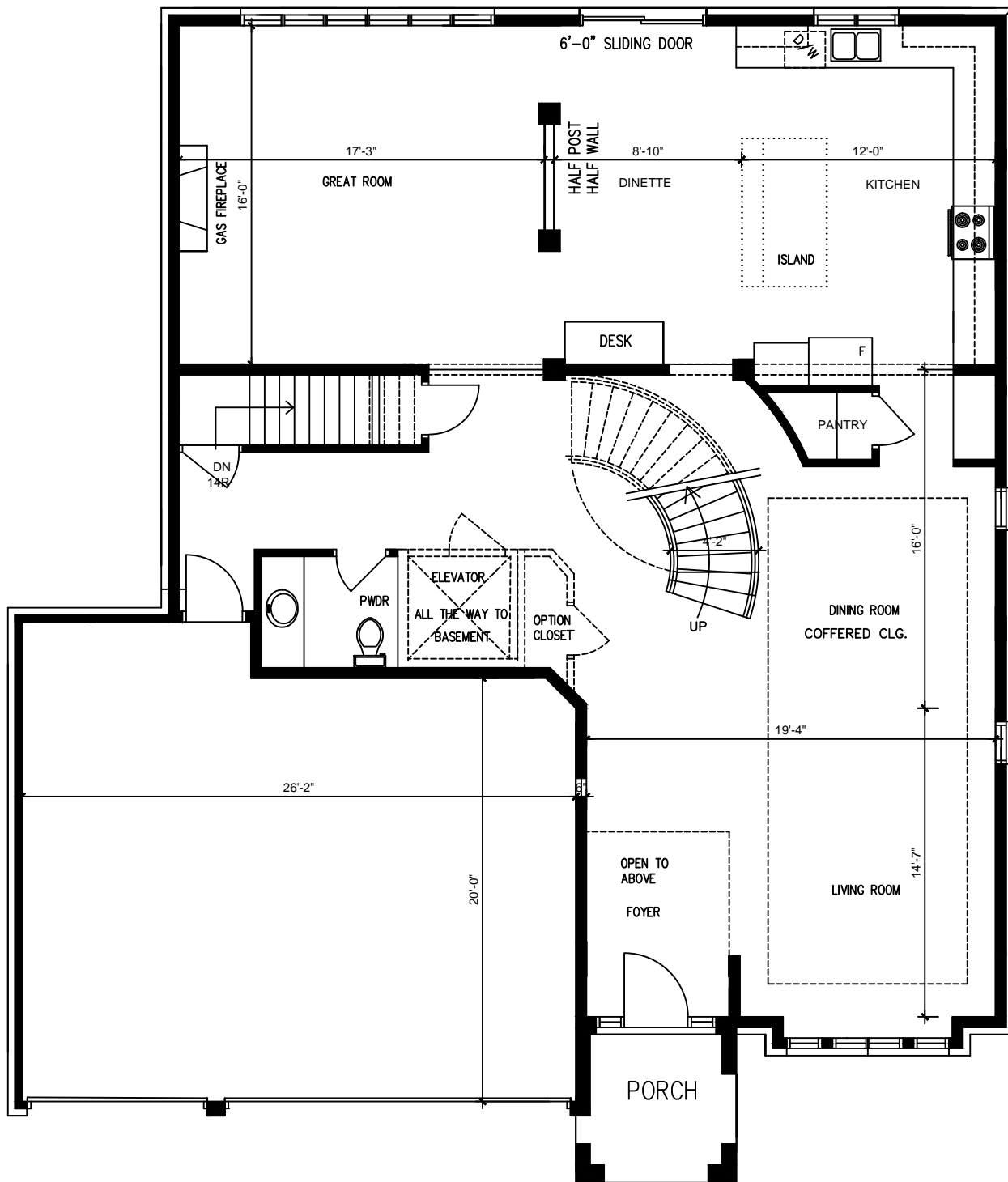
GROUND FLOOR PLAN 1622 S.F.
