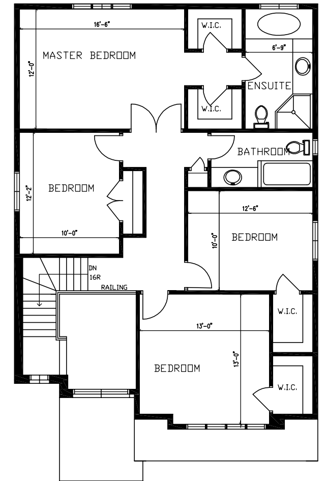
SECOND FLOOR 1238 S.F. INCLUDES OPEN TO ABOVE 90 S.F. TYPE "B"
