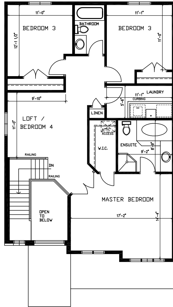
SECOND FLOOR 1221 S.F. INCLUDES OPEN TO ABOVE 127 S.F. TYPE "A"
