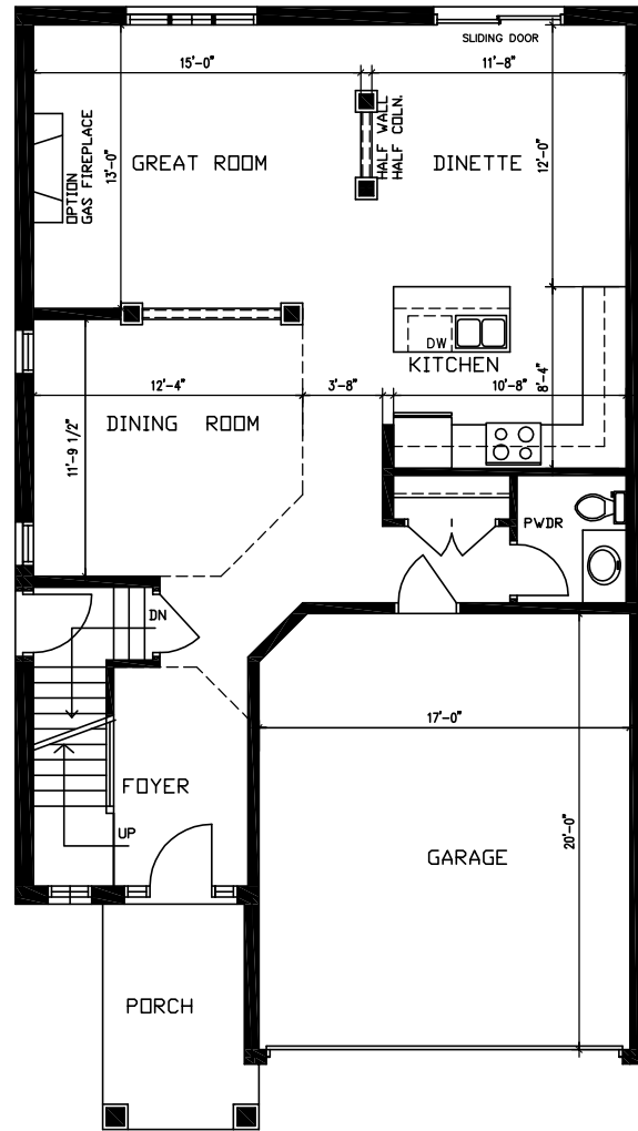
GROUND FLOOR 954 S.F. TYPE "A"
