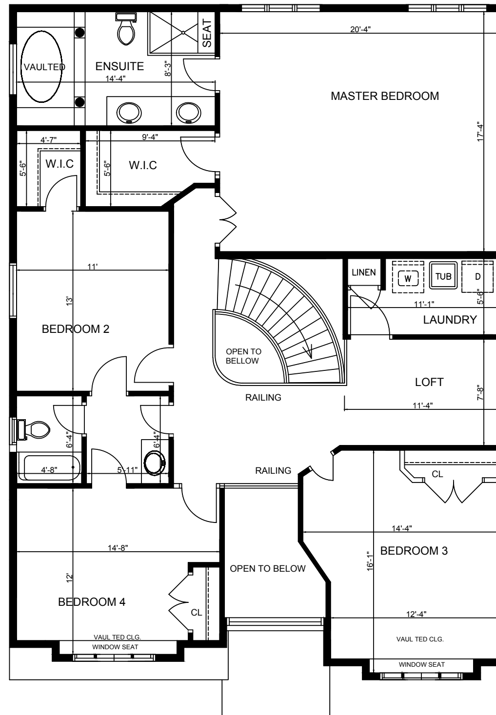
SECOND FLOOR 1845 s.f.
