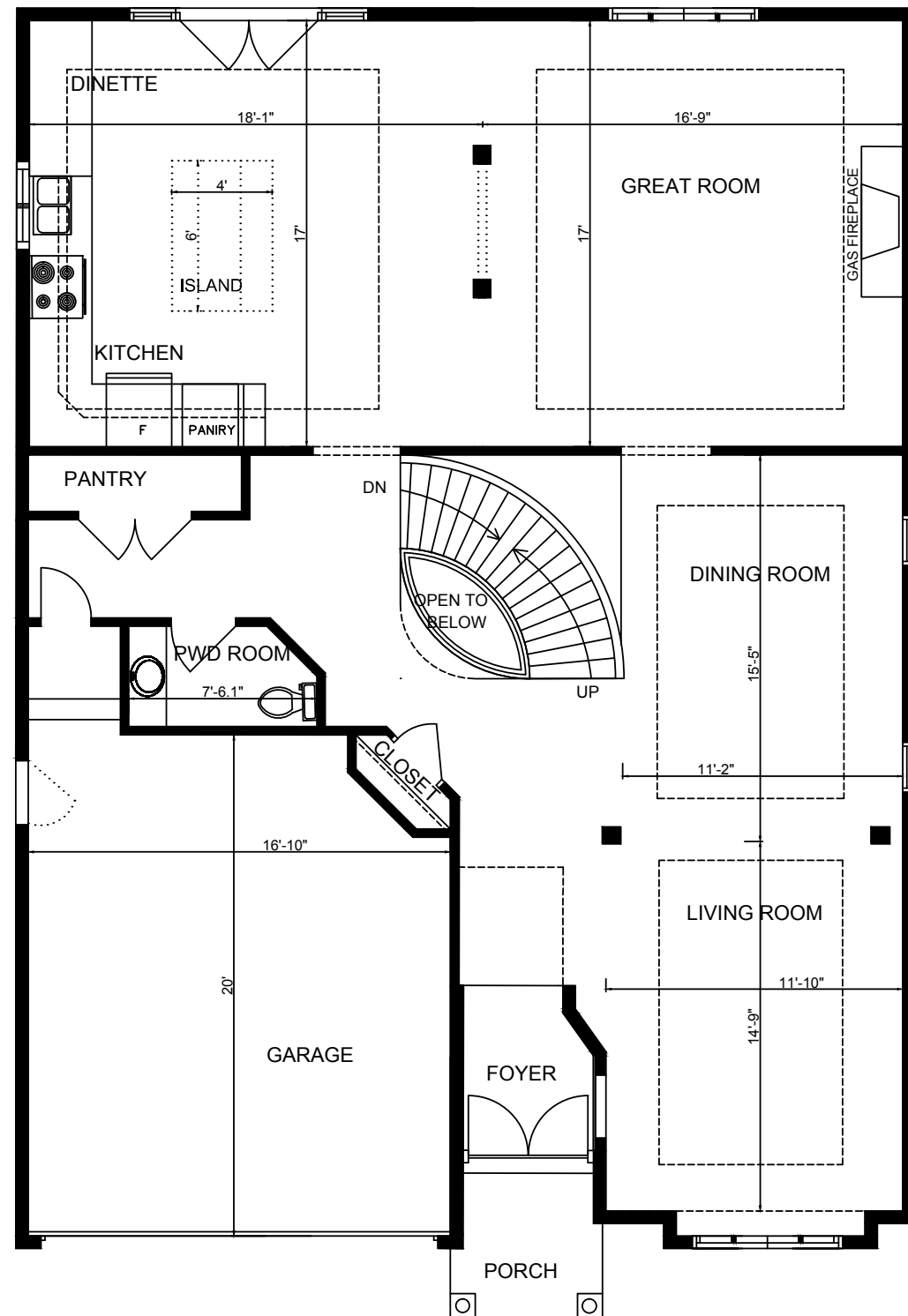
MAIN FLOOR 1497 s.f.
